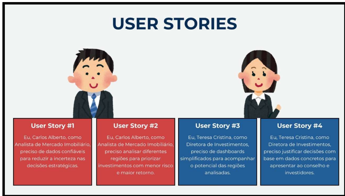
Figura 26 – User Stories.
